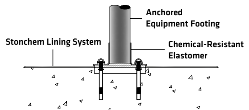
ANCHORED EQUIPMENT FOOTING
