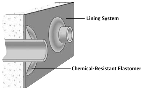
SEAL FOR PIPE PENETRATIONS
